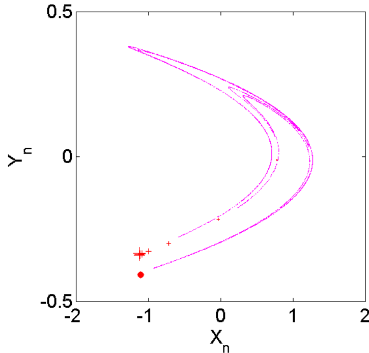
Seltsamer Attraktor: X_0 = -1.11, Y_0 = -0.408
