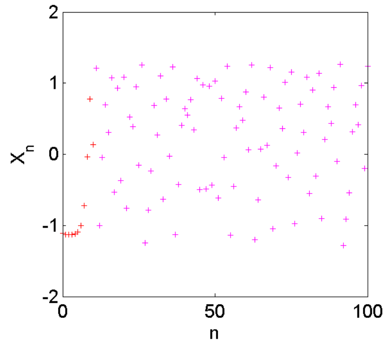
Seltsamer Attraktor: X_0 = -1.11, Y_0 = -0.408
