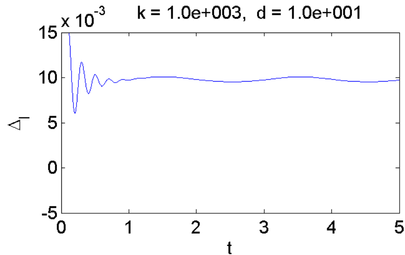
Steifes Pendel k = 1.0e+003 , d = 1.0e+001
