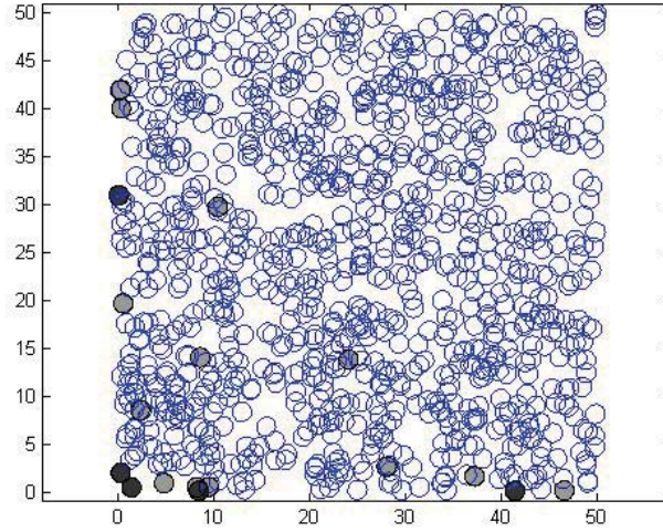
FIGURE 3. The lightly filled circles belong to the set \mathcal{T} generated by Algorithm 4.4 and the darkly filled circles are the elements which are minimal w.r.t. \preceq_D^u (see Example 4.20).
