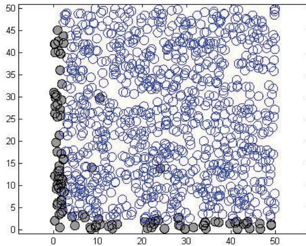
FIGURE 1. A randomly generated family of sets. The filled circles belong to the set \mathcal{T} generated by Algorithm 4.1.
