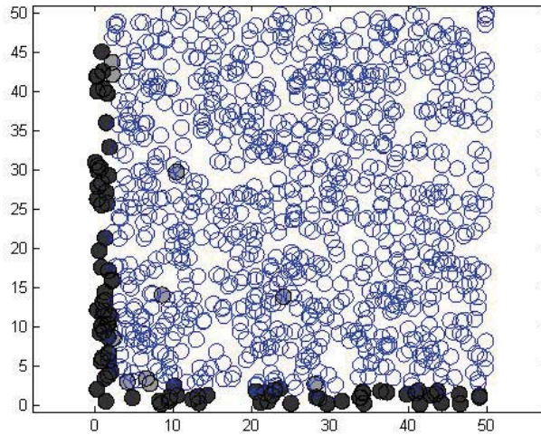
FIGURE 2. A randomly generated family of sets. The minimal elements w.r.t. \preceq_D^c are dark, the lighter sets belong to the set \mathcal{T} generated by Algorithm 4.2.
