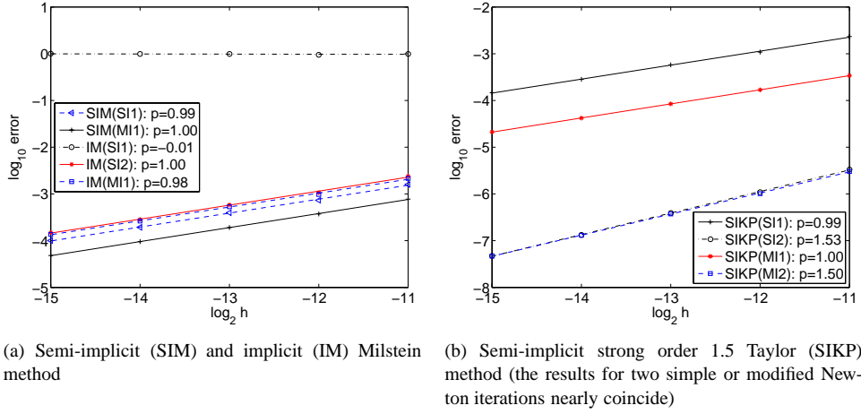
FIGURE 3. Error of several Taylor methods applied to (35) with up to two simple (SI) and modified Newton (MI) iterations
