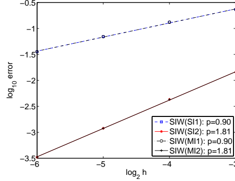
FIGURE 4. Error of the weak second order (semi-) implicit Platen method applied to (35) with one or two simple (SI) or modified Newton (MI) iterations (the results for one respectively two simple and modified Newton iterations coincide)
