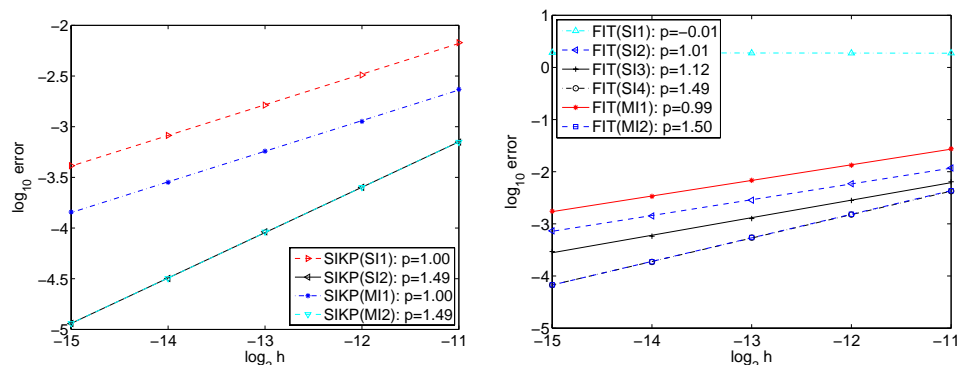
(a) Semi-implicit strong order 1.5 Taylor (SIKP) method (the results for two simple or modified Newton iterations coincide)
