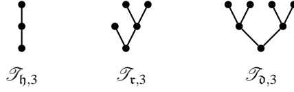
FIGURE 2. Minimal order trees with g(\tau) = 3 . The sets \mathcal{T}_{g,3} consist of all such trees with only stochastic nodes.
